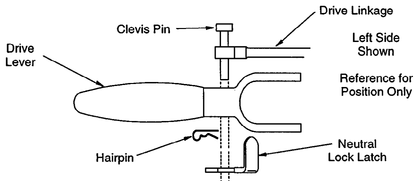
FIG. 11 DRIVE LEVER HARDWARE LOCATION
