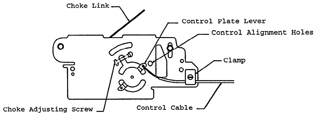
FIG 4 17 HP KAWASAKI SPEED CONTROL (THROTTLE CABLE HOOK-UP)
