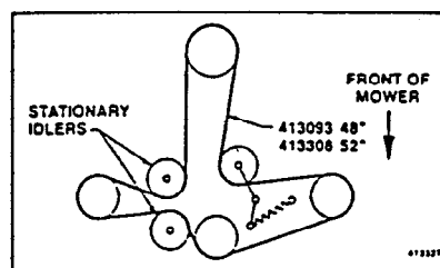
Part No. 413327 LOCATION: Top of Cutter Deck Under Center Belt Shield (48" & 52" Decks)
