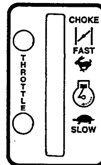
17 HP Kawasaki Part No. 323409
