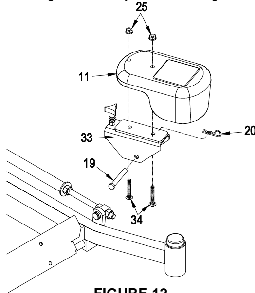
FIGURE 12 REMOVABLE WEGHT INSTALLATION
